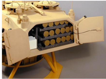
1:4 Scale LCTS 90mm Turret: ammunition compartment
