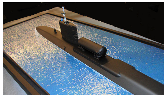
1:100 scale Swiftsure class submarine with DDH
