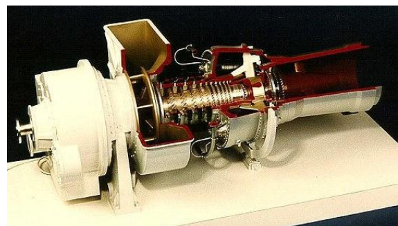
1:4 scale Industrial Gas Turbine
