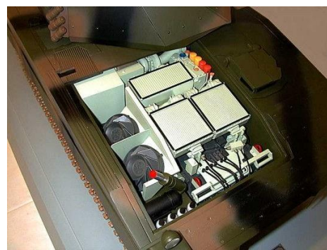
1:10 Scale Warrior with CV8 Powerpack
