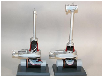
Sales demonstrator valve models
