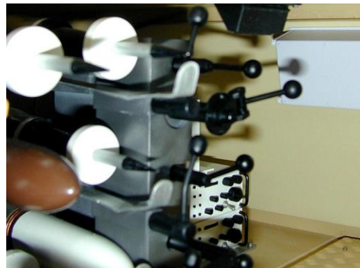
1:4 Scale LCTS 90mm Turret: Ammunition loading system
